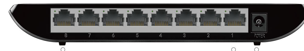
8 10/100/1000Mbps Ethernet Ports Power Socket
